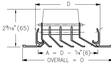
LV1/DV1 c/w 1" o/c DIRECTIONAL VANES
