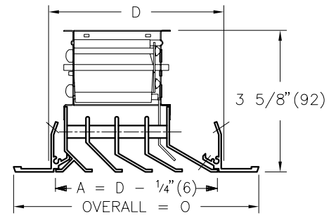
LV1/3 c/w OPPOSED BLADE DAMPER.
