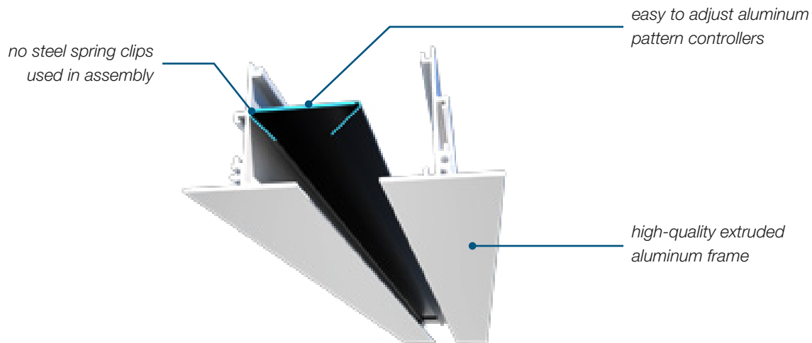
Model CF – Custom Flow linear diffuser with MRI option
