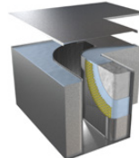
ERMT, ERMTX Film-lined Elbow & Extended Casing Silencers
