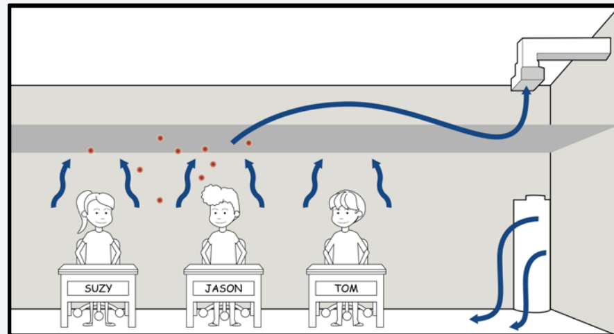
In a displacement system the sneeze particles (red) are pushed up and out of the breathing zone.
